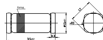
SOD-80 Quadro-melf
