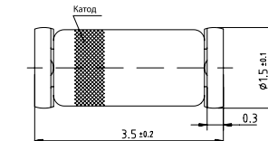
SOD-80 Mini-melf
