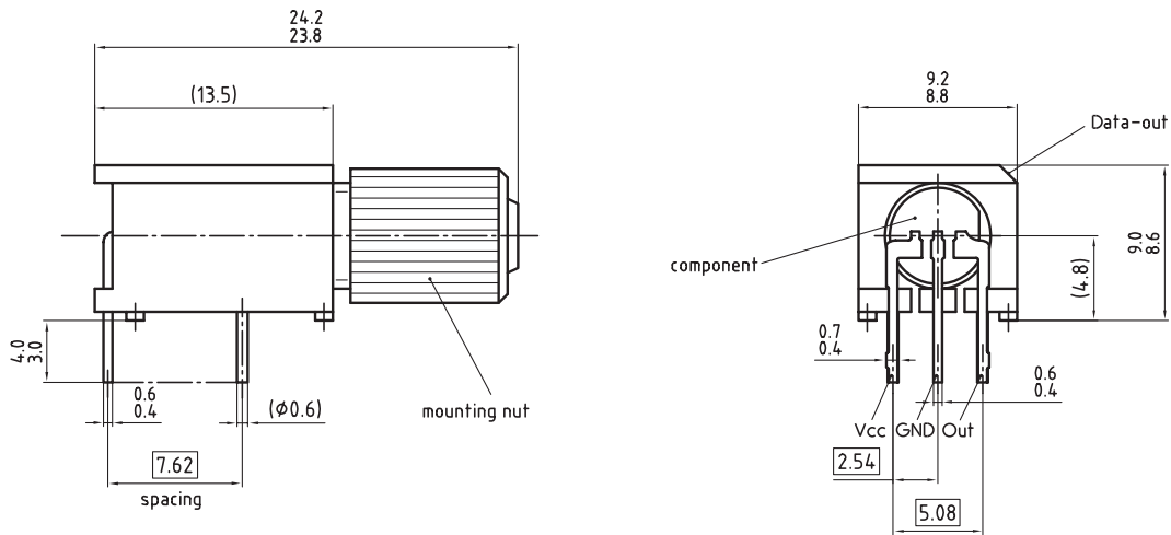
Figure 2. SFH551/1-1
