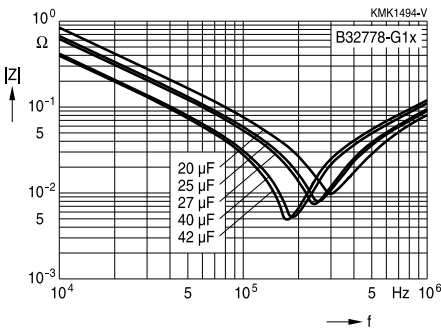
Impedance Z versus frequency f (typical values)
