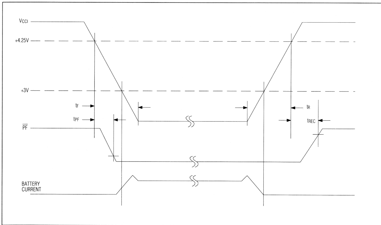
Figure 1. Power-Down/Power-Up Conditions
