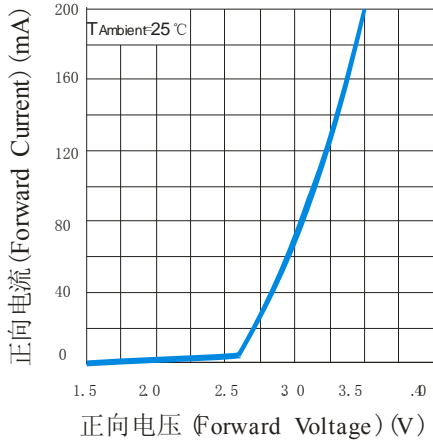
Volt-Ampere Characteristics
