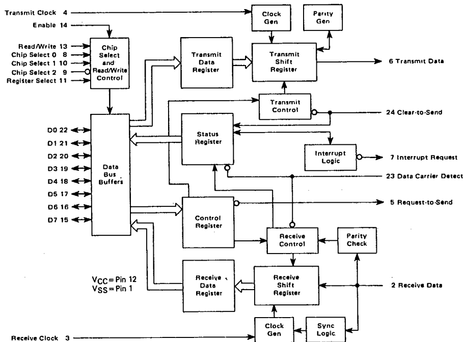
87D 09451 DT-75-37-05 FIGURE 9 - EXPANDED BLOCK DIAGRAM
