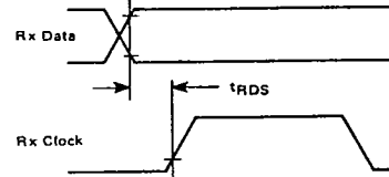
FIGURE 4 — RECEIVE DATA SETUP TIME (+1 Mode)
