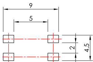
SMD REFLOW PATTERN
