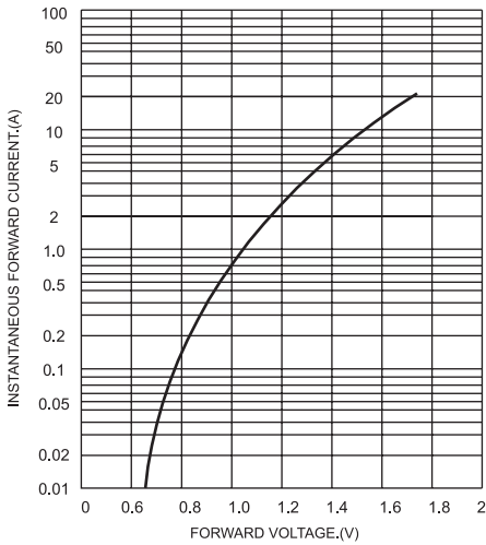
FIG.3-TYPICAL FORWARD CHARACTERISTICS
