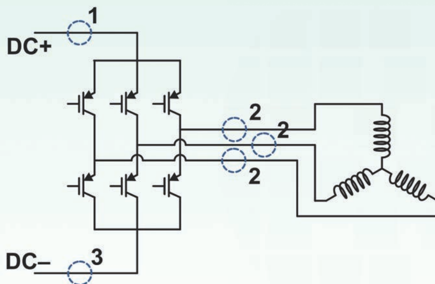
Figure 5: Typical current sensing locations in motor controller applications
